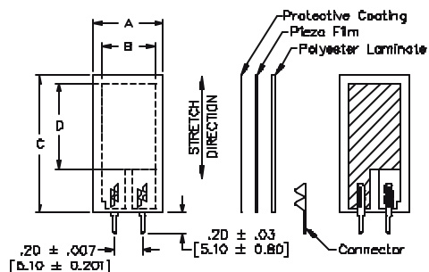
LDT0-028K (with crimped-on solder tabs)
